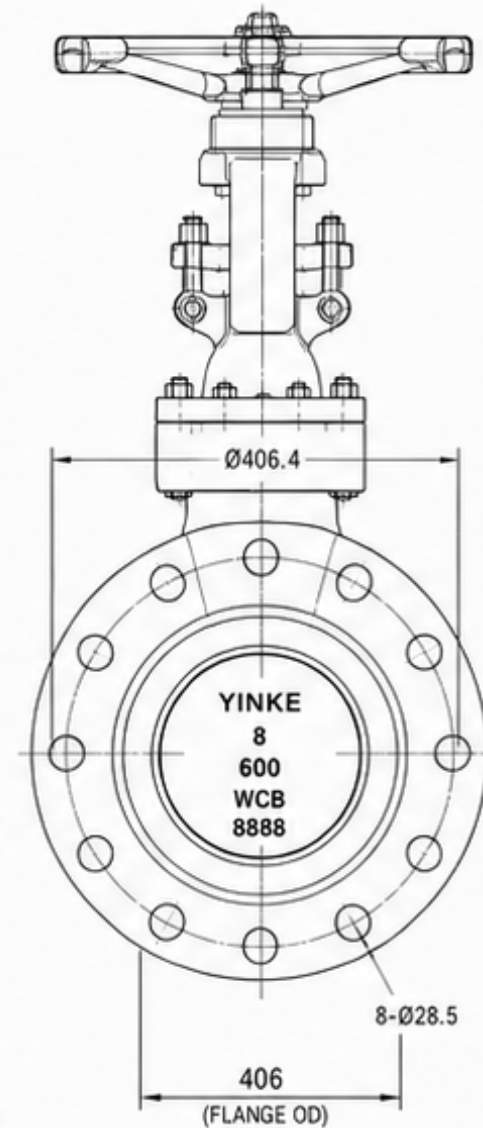
B. END VIEW (RF FLANGE INTERFACE)
