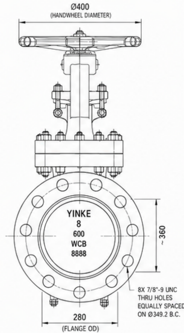
B. END VIEW (RF FLANGE INTERFACE)
